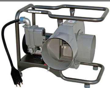
Custom Small Portable 6" Pressure Blower Designed for Hazardous Location Ventilation
